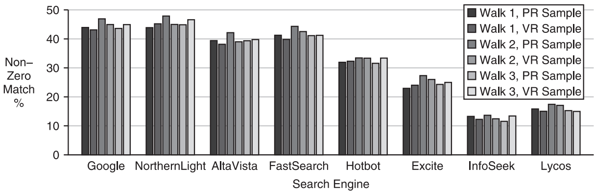
Fig. 7. Non-zero matches for the three walks.
